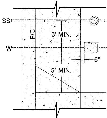
TYPICAL LAYOUT
