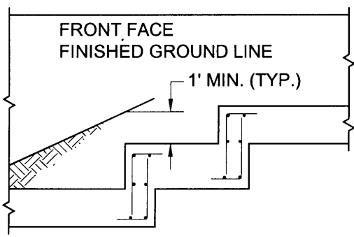
FOOTING STEP ELEVATION
