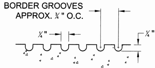
GROOVING DETAIL
