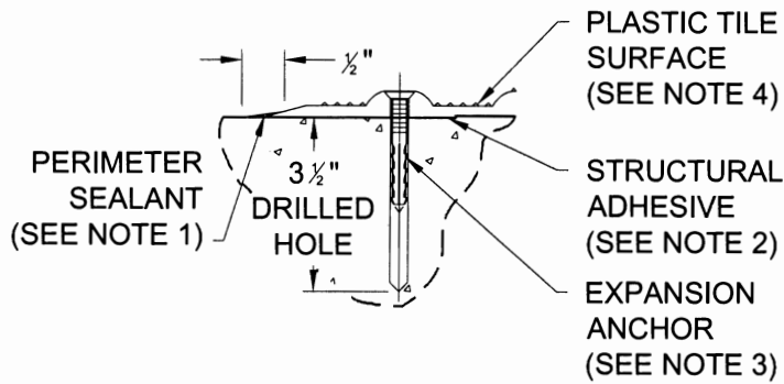
SURFACE APPLIED TILE INSTALLATION
