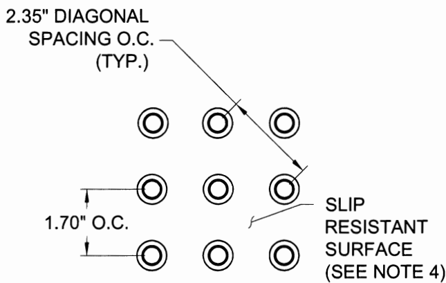
RAISED TRUNCATED DOME PATTERN
